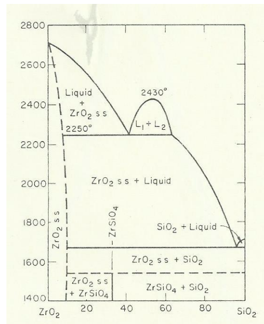
Figure 7. Phase diagram of ZrSiO 4 .
