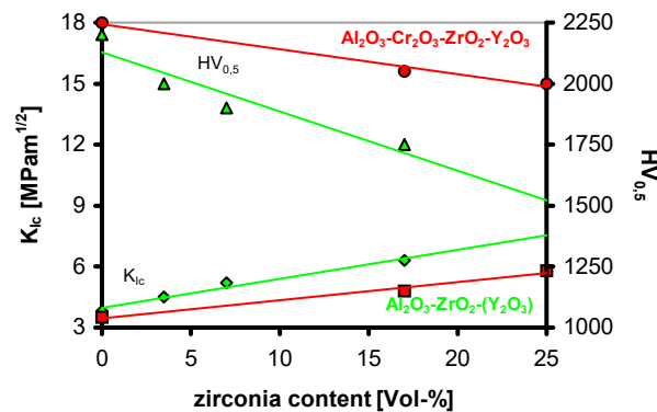
Figure 28. Fracture toughness and hardness within the system Al_2O_3-ZrO_2:Y-Cr_2O_3 .
