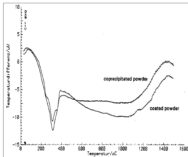
Figure 15. DTA-analysis of coprecipitated and coated yttria-zirconia composites.
