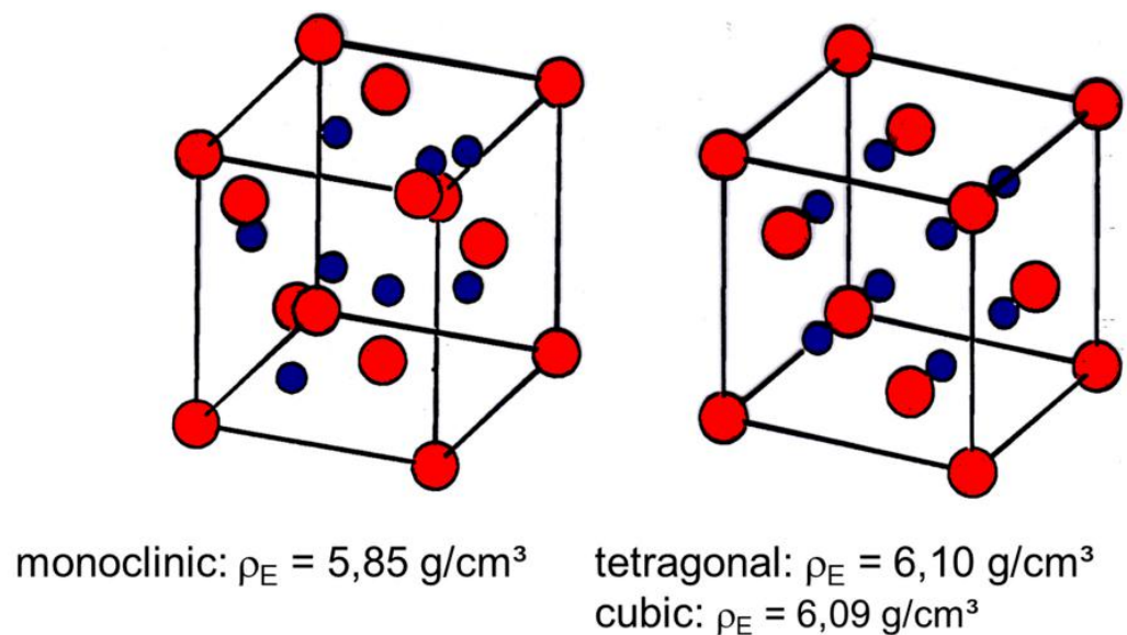
Figure 5. Orientation of the Zr-ions in the monoclinic and tetragonal lattice.
