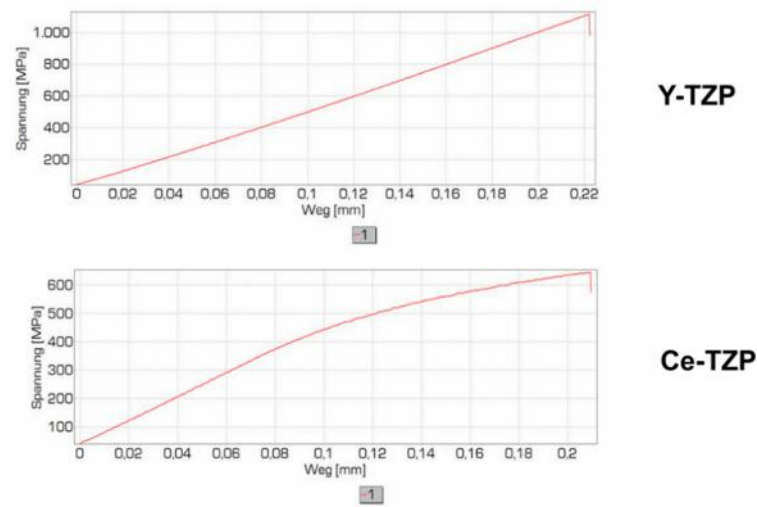
Figure 35. Stress-strain behaviour of Y-TZP and Ce-TZP.
