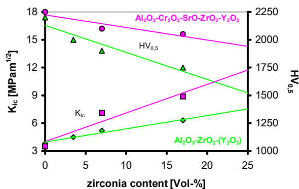
Figure 29. Fracture toughness and hardness in the system Al_2O_3-Cr_2O_3-ZrO_2-Y_2O_3-SrO .
