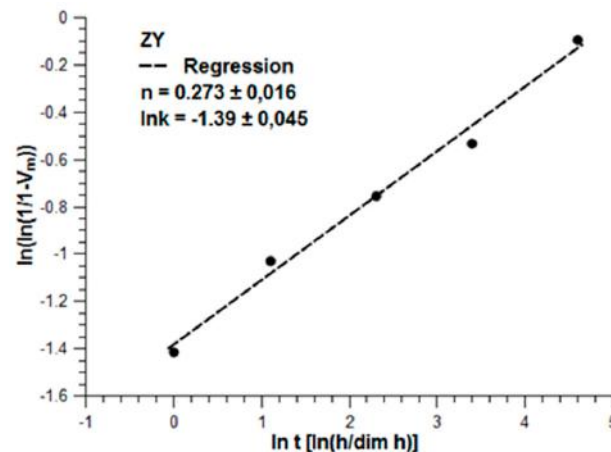
Figure 24. Increase of monoclinic phase according to Mehl-Avrami-Johnson-kinetics.
